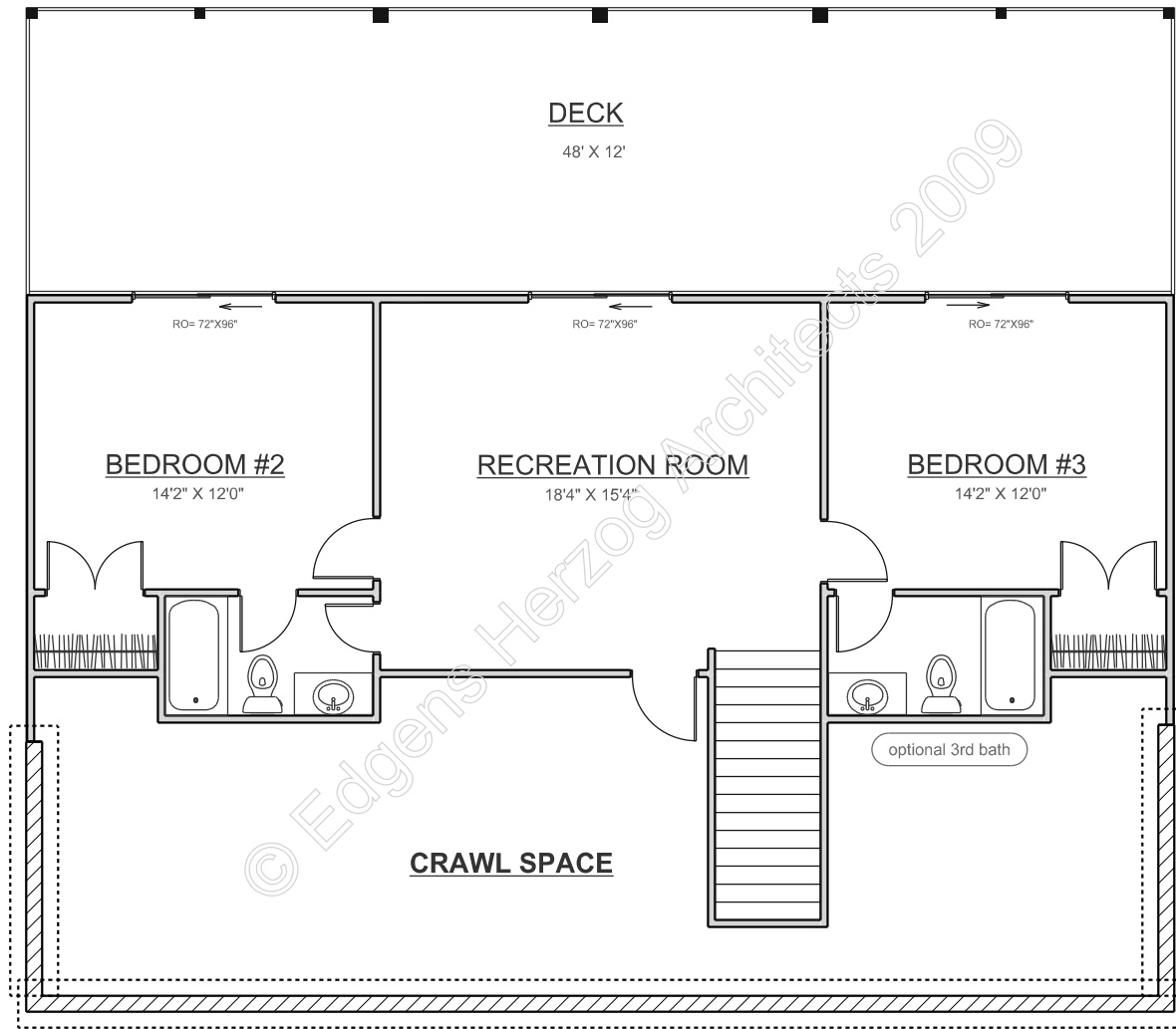
BASEMENT PLAN
